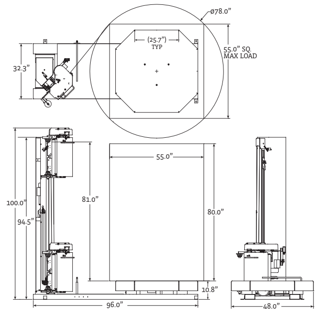
Flex HPD - Dimensions - Inches
